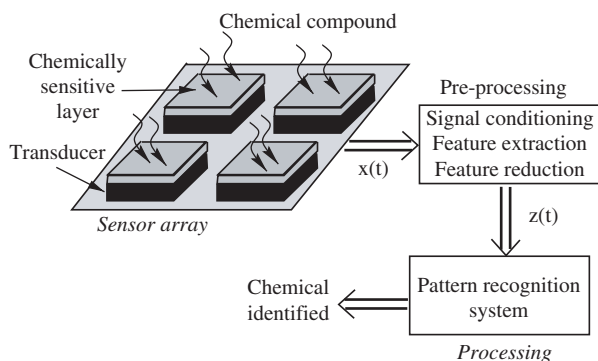
Figure 1. Electronic nose block diagram.
