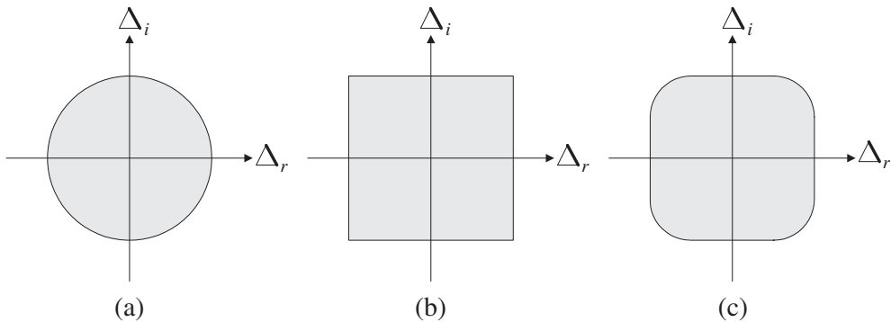
Figure 8.9 Different uncertainty regions for the case of a scalar error \Delta , where \Delta_r = \text{Re} \{ \Delta \} and \Delta_i = \text{Im} \{ \Delta \} . (a) estimation Gaussian noise, (b) quantization errors, and (c) combined estimation and quantization errors.
