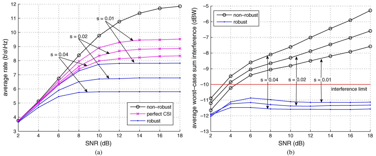
Fig. 3. Comparison of the robust and non-robust power allocation for a single SU in SISO frequency-selective channels; N = 16 , I^{\text{ave}} = -10 dB, d = 3 . (a) Average information rate. (b) Average worst-case sum interference.
