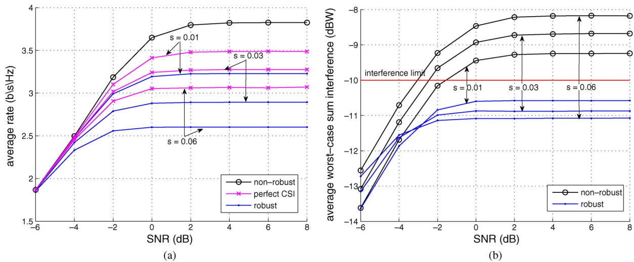
Fig. 4. Comparison of the robust and non-robust precoding for a single SU in MIMO channels; M = N = 4 , I^{\text{ave}} = -10 dB, d = 3 . (a) Average information rate. (b) Average worst-case sum interference.
