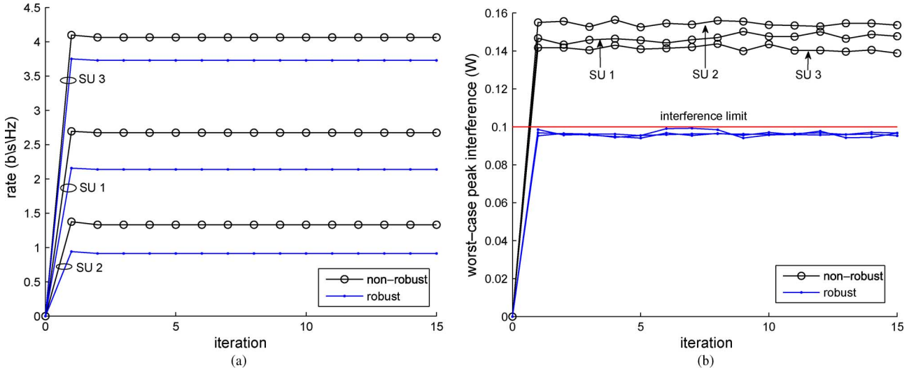
Fig. 8. Comparison of the robust game \hat{\mathcal{G}}_{\text{mimo}} and non-robust game \mathcal{G}_{\text{mimo}} using the simultaneous MIMO RICA; M = N = 2 , I^{\text{ave}} = 0.1 (-10 dB), d = 2.5 , SNR = 3 dB, s = 0.04 . (a) Iteration of the SUs' rates. (b) Iteration of the SUs' worst-case peak interference.
