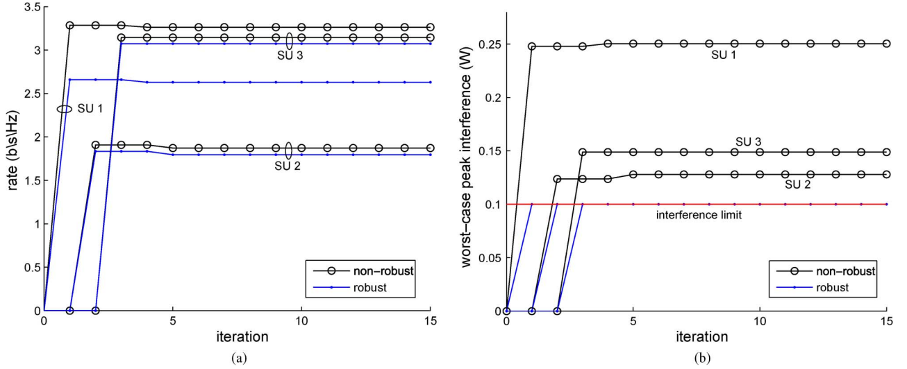
Fig. 7. Comparison of the robust game \hat{\mathcal{G}}_{\text{siso}} and non-robust game \mathcal{G}_{\text{siso}} using the sequential SISO RICA; N = 8 , I^{\text{ave}} = 0.1 (-10 dB), d = 2 , SNR = 3 dB, s = 0.04 . (a) Iteration of the SUs' rates. (b) Iteration of the SUs' worst-case peak interference.
